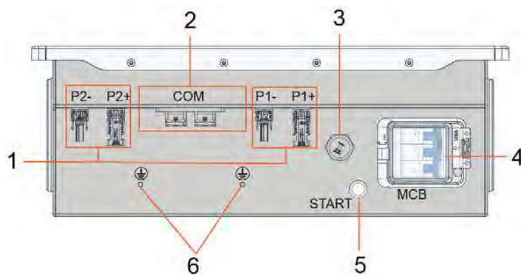
Figure 2-3 Bornes
