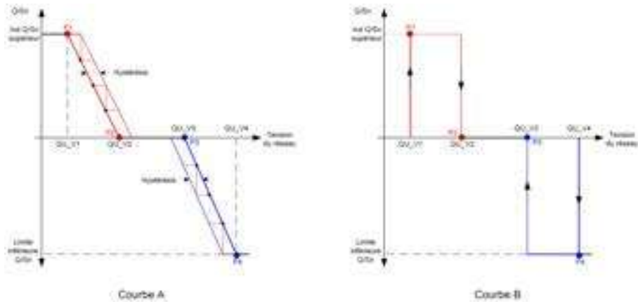
figure 8-28 Courbe Q(U)
