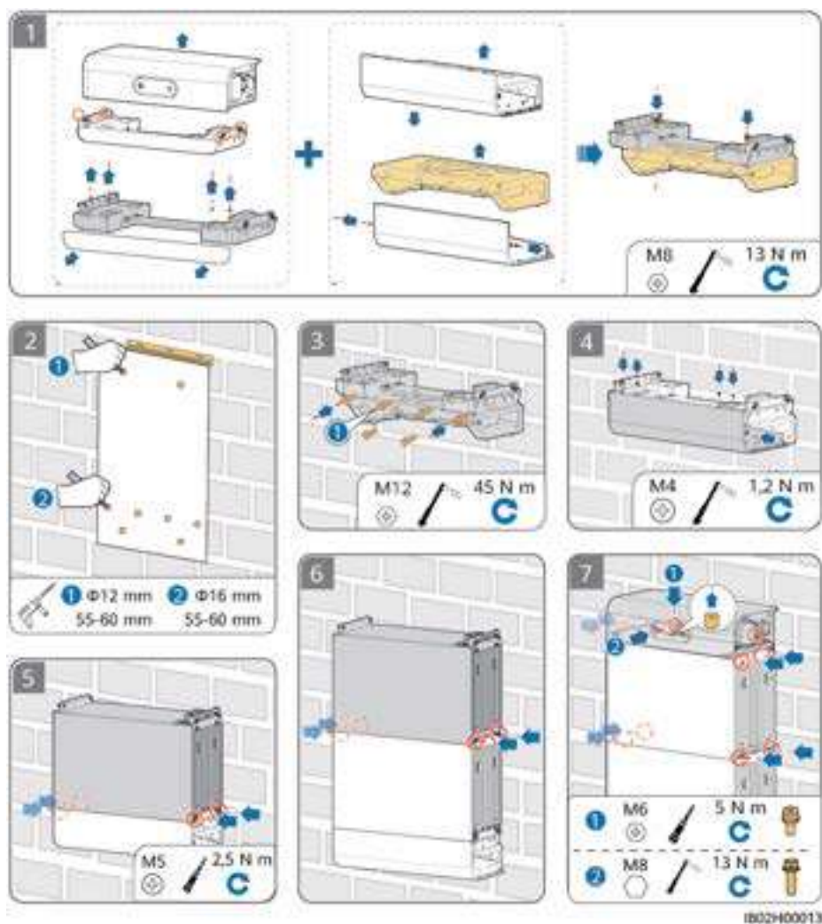
Figure 4-6 Montage mural
