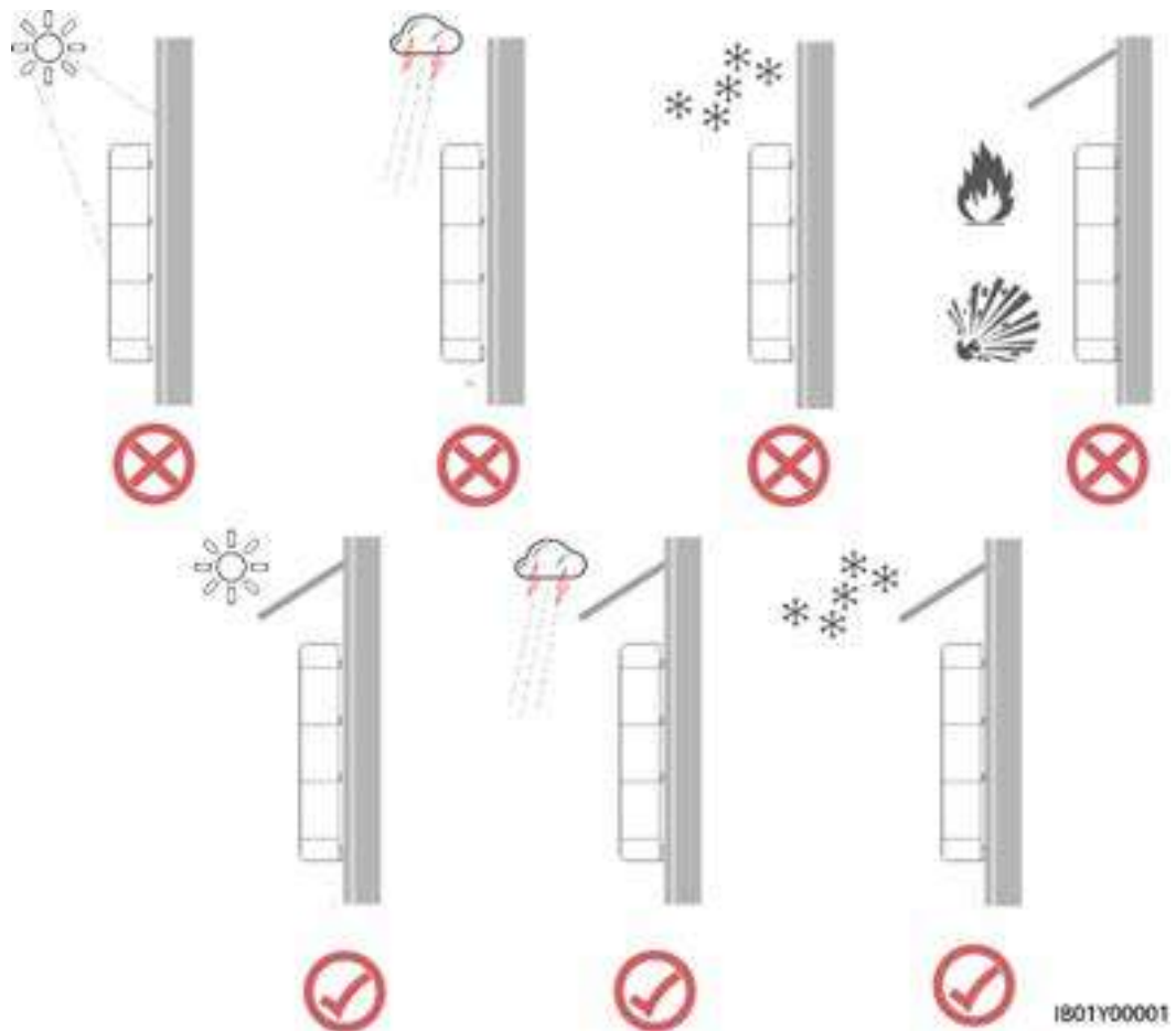
Figure 1-3 Installation environnement
